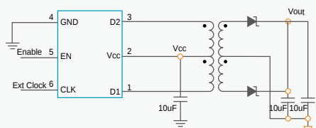
Figure 2.Simplified Schematic
